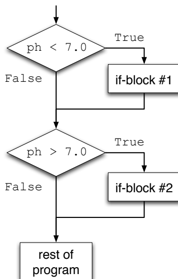
Figure 6.4: if statement
